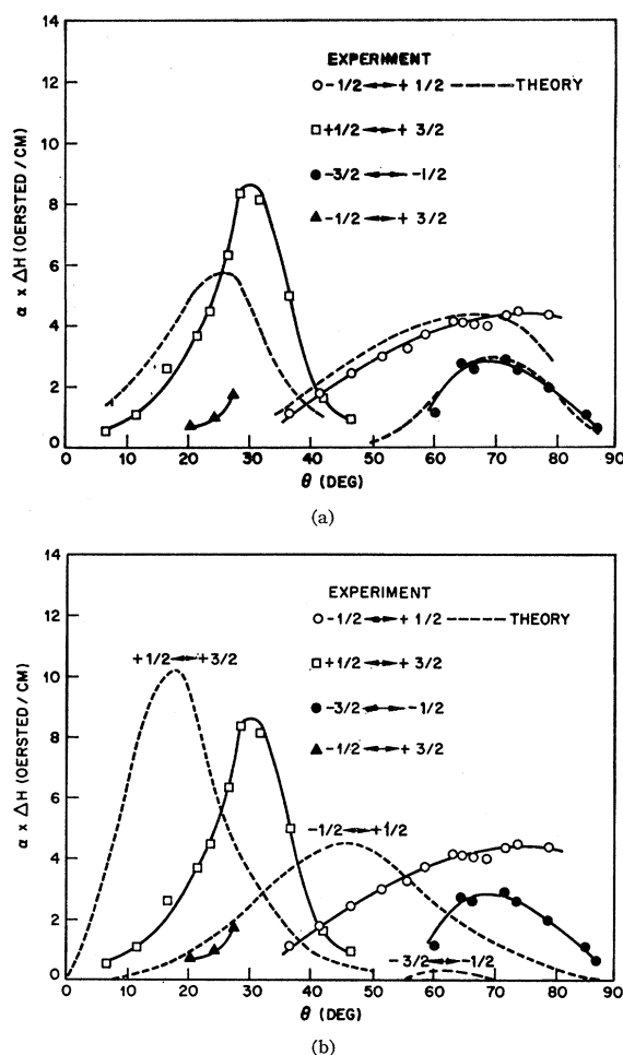
Fig. 4. Comparison of the quadrupolar [Fig. 4(a)] and dipolar [Fig. 4(b)] theories with the experimental angular dependence of the absorption coefficient multiplied by the linewidth in 0.08% ruby. To normalize the theoretical curves the computed point for \frac{1}{2} \leftrightarrow -\frac{1}{2} transition was set equal to the experimental value for \theta=70^\circ in Fig. 4(a) and \theta=55^\circ in Fig. 4(b).
