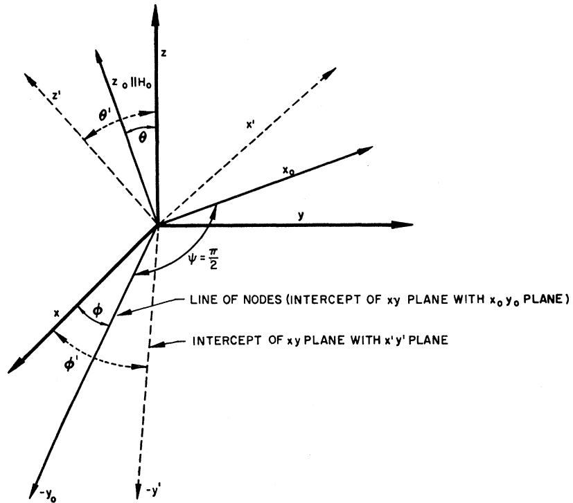
FIG. 1. x, y, z —crystalline coordinate system. x_0, y_0, z_0 —laboratory coordinate system. x', y', z' —diagonal coordinate system. \theta' = \sin^{-1}[(g_1/g)\sin\theta] , \varphi' = \sin^{-1}[(g_x/g_1)\sin\varphi] . Direction of H_0 in the xyz system is specified by the Eulerian angles \theta, \varphi ; since the choice of x_0, y_0 is arbitrary, the third Eulerian angle is taken as \psi = \pi/2 without loss of generality.
